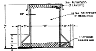
Series 20 Utility set support
